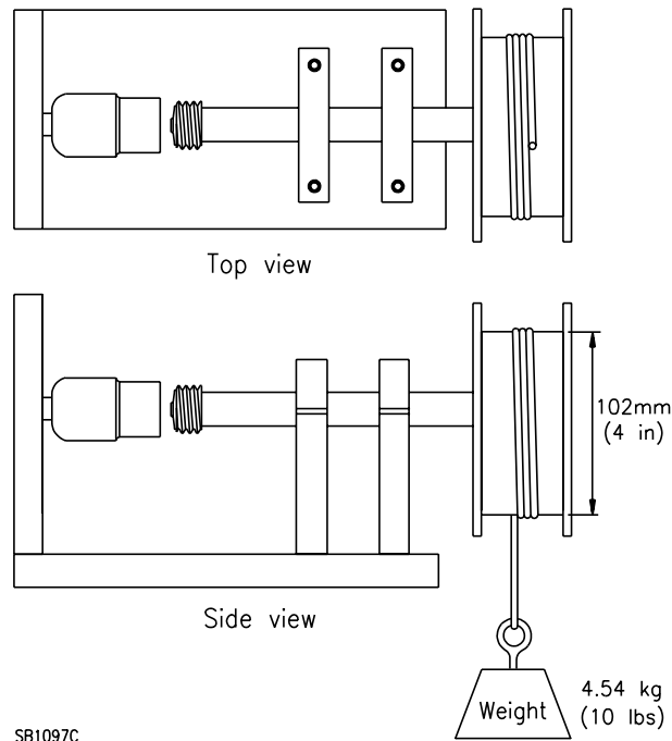
Figure 19.27.1 Medium-base lampholder mounting torsion test apparatus
