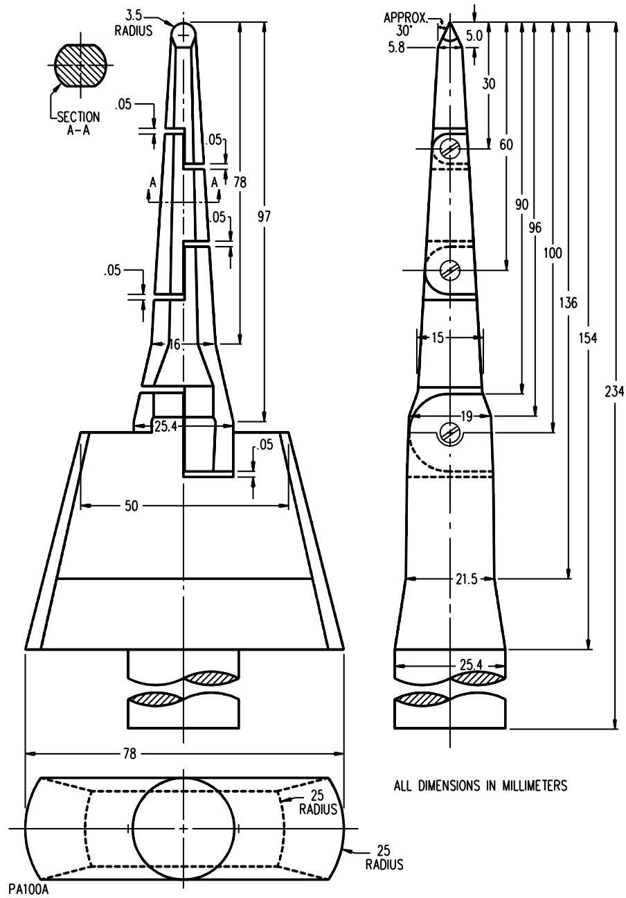
Figure 19.22.1 Articulate probe with web stop
