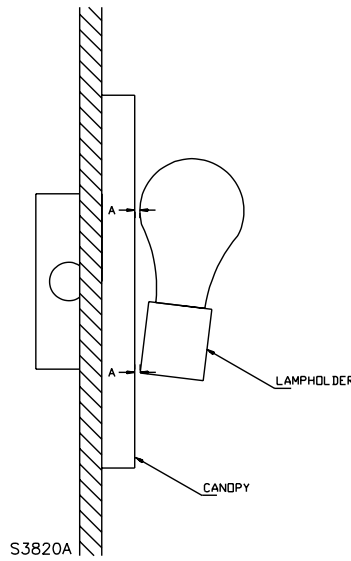
Figure 7.2.3.1 Minimum lamp spacings for wall-mounted luminaires
