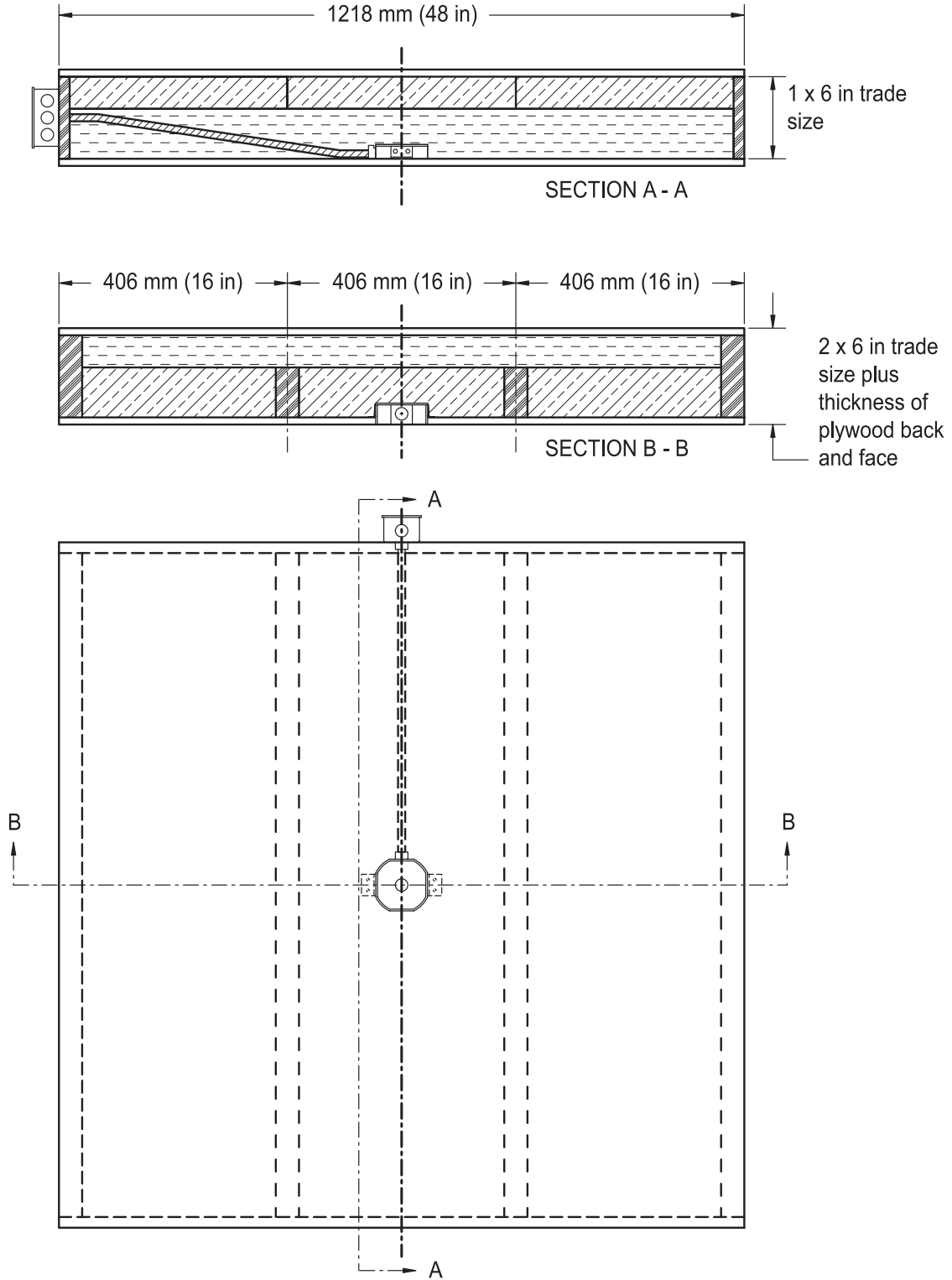
Figure 19.10.1 Surface ceiling temperature test apparatus
