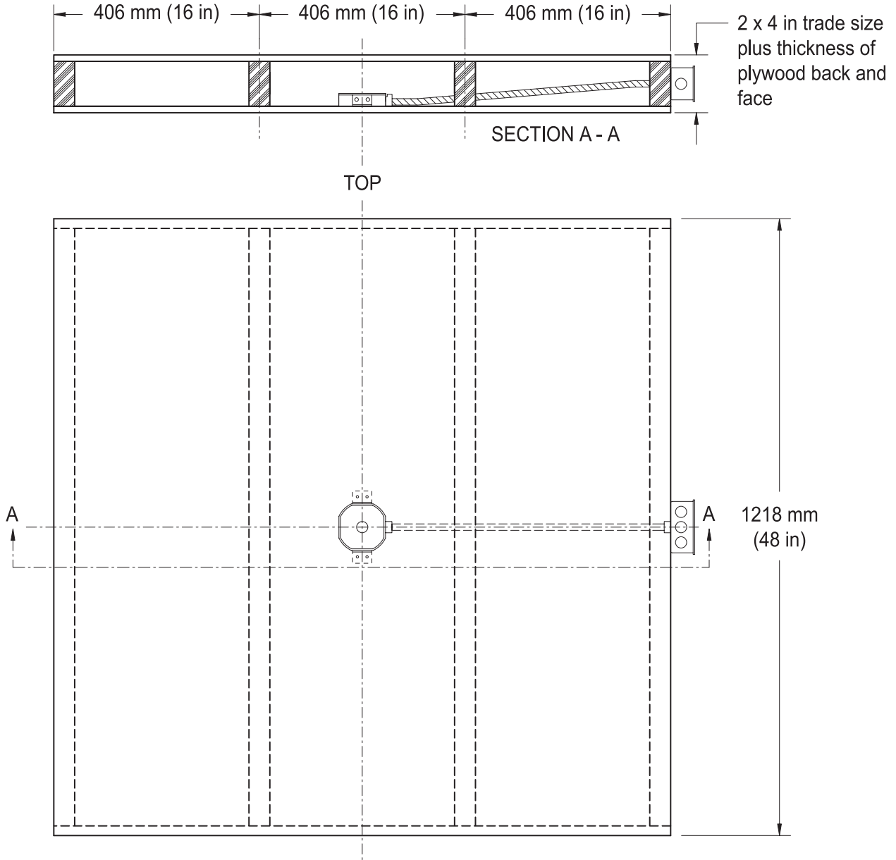
Figure 19.11.1 Test wall apparatus — wall surface luminaires
