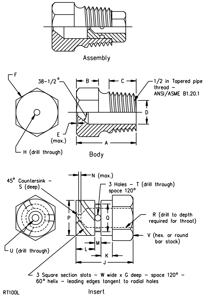
Figure 19.17.2 Spray head
