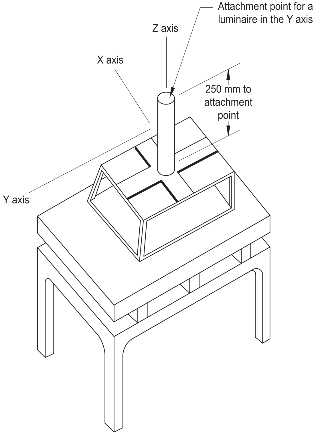
Figure 19.34.1 (MEX) Vibration table
