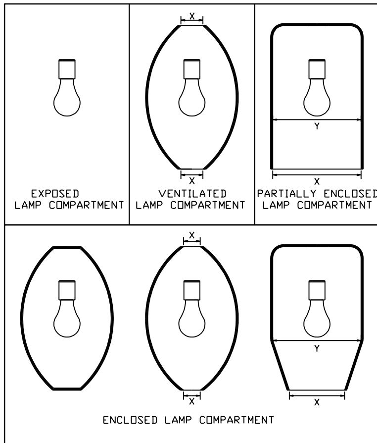
Figure 7.2.1.1 Temperature-test-exempt lamp compartment definitions (See Clause 7.2.1.4.)
