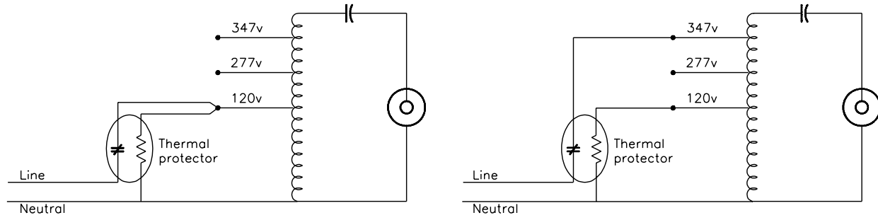
Figure 11.5.1.2 Wiring diagrams for an HID luminaire with a multi-tap autotransformer ballast and thermal protector with a 120 V integral heater
